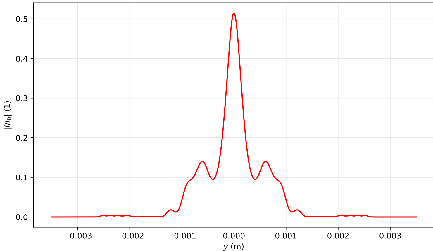
Intensity profile I(x=0, y, z=1.672)/I_0 , P_{in}=7.5P_{cr} , artificial time
